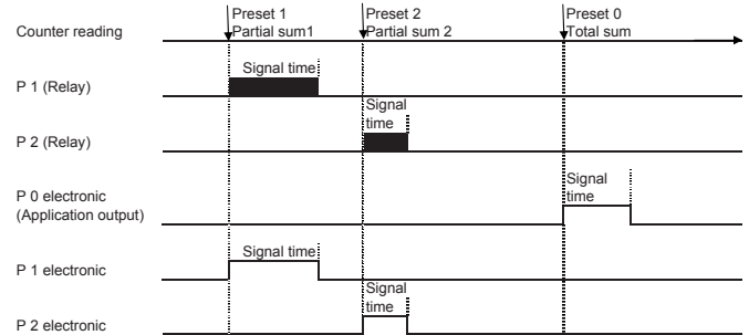
Coincidence signals P 0/Total Sum (F10), P 1/Partial sum 1 (F11), P 2/Partial sum 2 (F12) monostable
