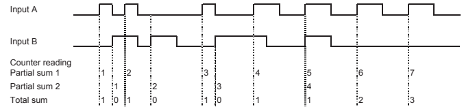
Adding/Subtracting (F1= A S r)
